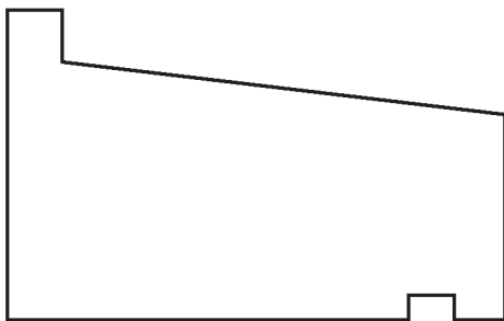
DRIP CAP 1-7/16 x 2-3/8 CEDAR & FIR
