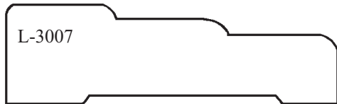
L-3007 MOULDED 5/8 x 2-3/8 POPLAR
