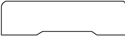
BULL NOSED 11/16 x 2-1/2 VG HEM & VG FIR
