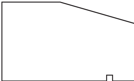
WINDOW SILL 1-3/8 x 2-3/8 CEDAR & F/J PRIMED CEDAR
