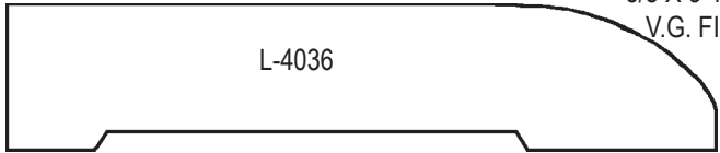
SANITARY BASE STYLE "A" 7/8 X 2-1/4 HEM
