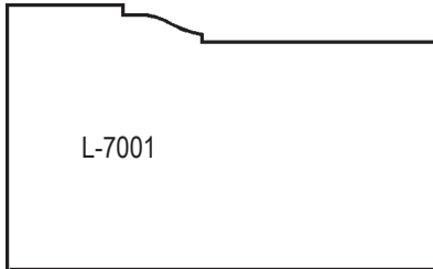
BRICK MOLD 1-1/4 X 2 SOLID HEM & F/J PRIMED
