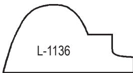
CHAIR RAIL 5/8 X 1-5/16 V.G. FIR
